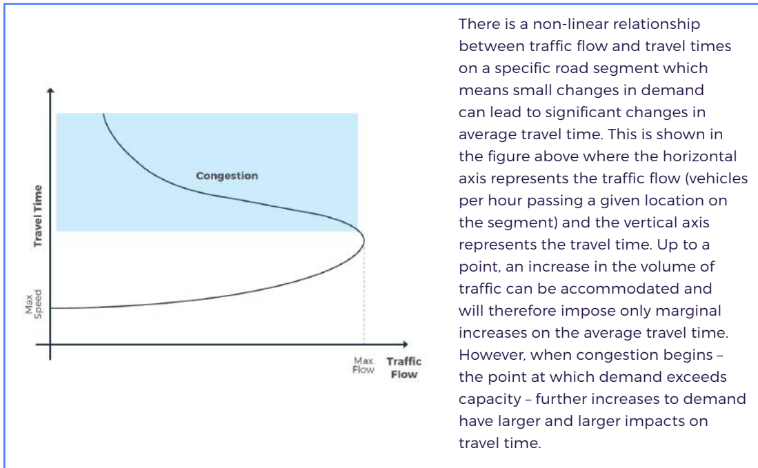
Figure B3-1: Non-linear relationship between traffic flow and travel time
