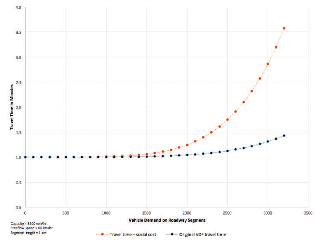
Figure B2-1: Travel time with original VDF and MSC VDF
